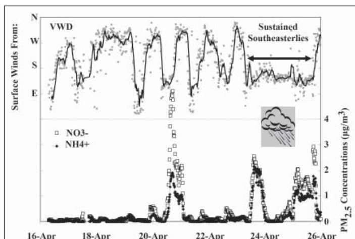
Figure 1. Time history of vector wind direction (VWD) and particulate-phase nitrogen species concentrations from 16-26 April 2006 at the core site in RMNP. A major precipitation event is indicated.
