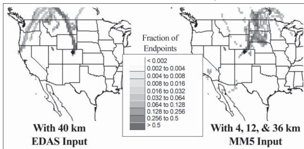
Figure 4. Frequency of contact with geographical grid cells using 5-day back trajectories for air masses arriving at the RoMANS core site for the 24-hour period on 24 April 2006. Back trajectories were calculated using the NOAA HYSPLIT model with 40 km horizontal resolution EDAS data (left) and with nested grid (4, 12, and 36 km) MM5 data (right).
