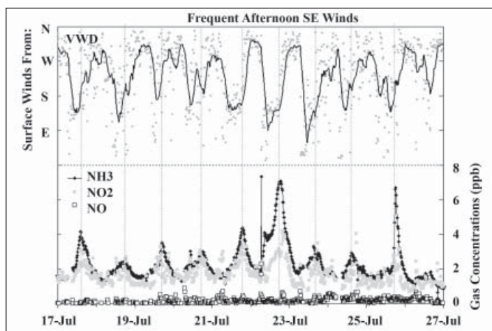
Figure 2. Time history of vector wind direction (VWD) and gas-phase nitrogen species concentrations from 17-27 July 2006 at the core site in RMNP. Daily peaks in \text{NH}_3 and \text{NO}_2 concentrations often follow changes to southeasterly winds as indicated.
