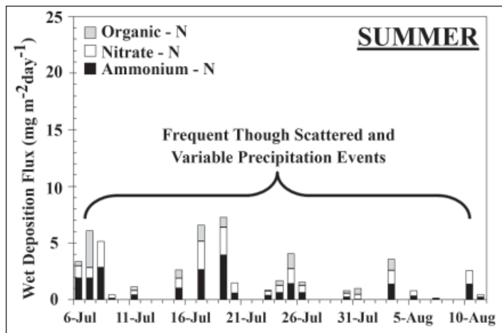
Figure 3. Timeline of wet deposition nitrogen fluxes based on 24-hour precipitation samples (08:00-08:00 MST) during the spring and summer RoMANS campaigns.
